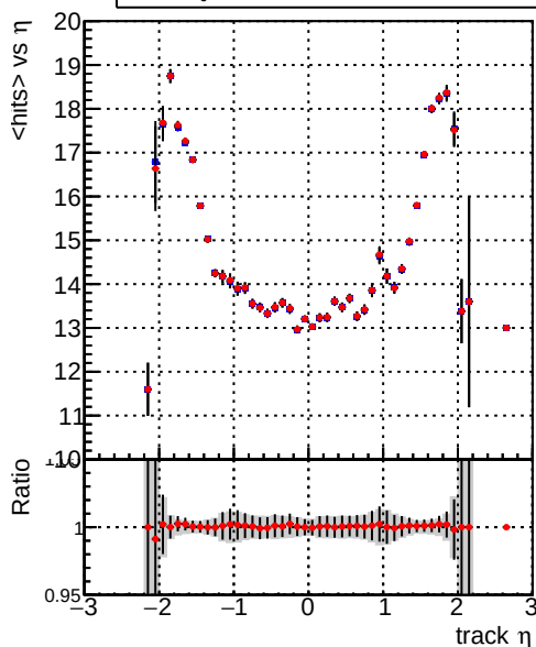
mean hits — DQM_V0001_R000000001_Global_CMSSW_orig — DQM_V0001_R000000001_Global_CMSSW_allchi2
