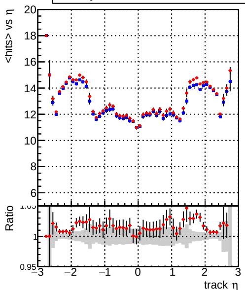
mean hits — DQM_V0001_R000000001_Global_CMSSW_orig — DQM_V0001_R000000001_Global_CMSSW_allchi2
