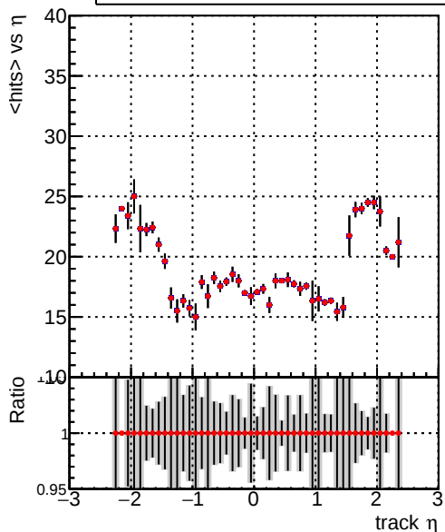
mean hits — DQM_V0001_R000000001_Global_CMSSW_orig — DQM_V0001_R000000001_Global_CMSSW_allchi2
