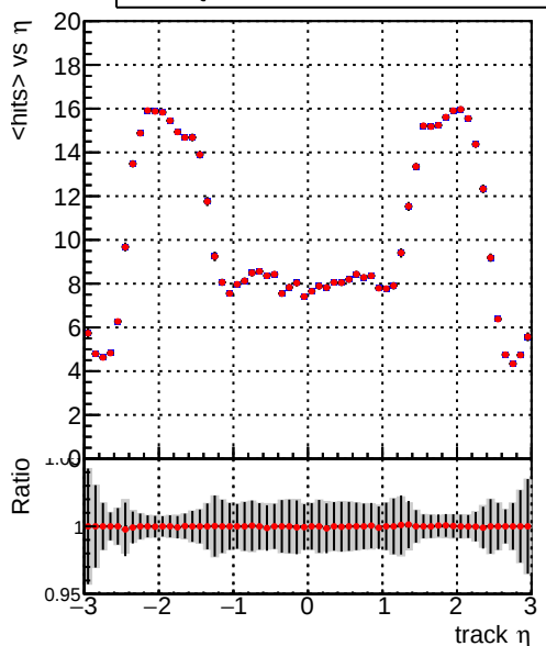
— DQM_V0001_R000000001_Global_CMSSW_orig — DQM_V0001_R000000001_Global_CMSSW_allchi2
