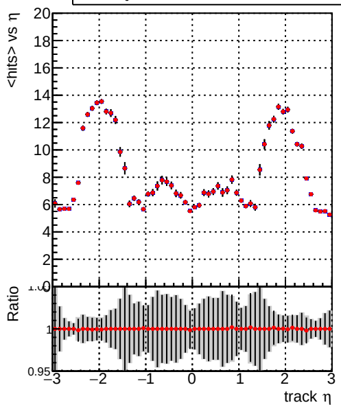
— DQM_V0001_R000000001_Global_CMSSW_orig — DQM_V0001_R000000001_Global_CMSSW_allchi2
