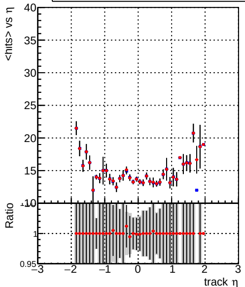
— DQM_V0001_R000000001_Global_CMSSW_orig — DQM_V0001_R000000001_Global_CMSSW_allchi2
