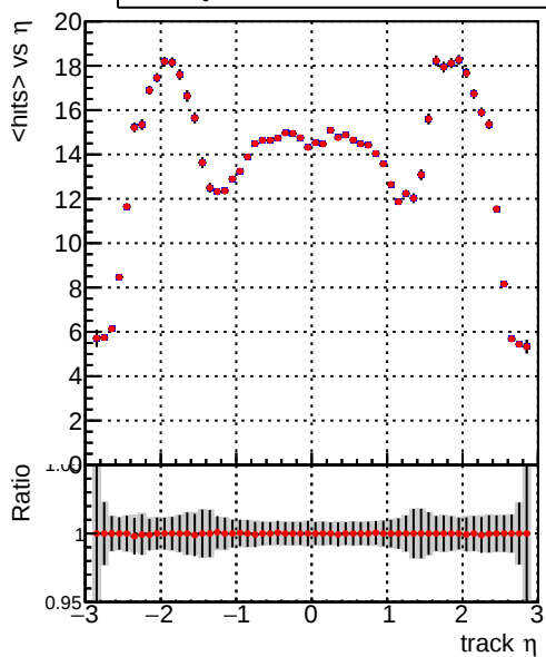
— DQM_V0001_R000000001_Global_CMSSW_orig — DQM_V0001_R000000001_Global_CMSSW_allchi2
