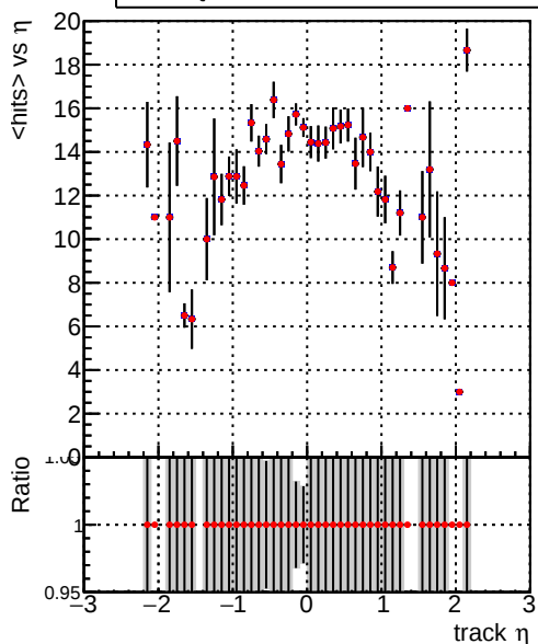
— DQM_V0001_R000000001_Global_CMSSW_orig — DQM_V0001_R000000001_Global_CMSSW_allchi2
