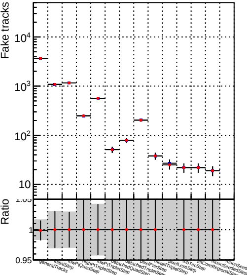
Number —●— DQM_V0001_R000000001_Global_CMSSW_allchi2
