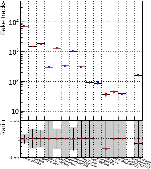
Number —●— DQM_V0001_R000000001_Global_CMSSW_allchi2
