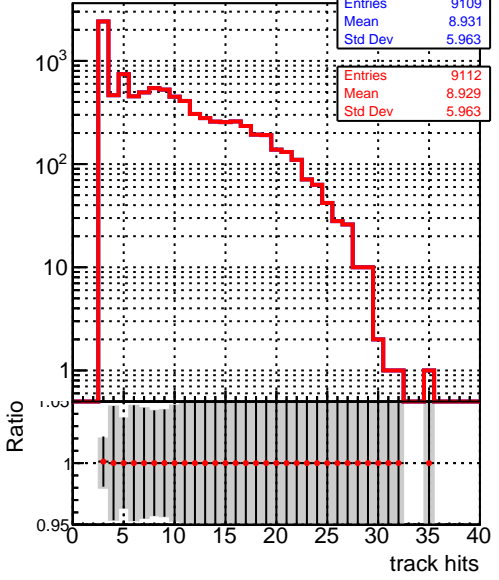
mean hit — DQM_V0001_R000000001_Global_CMSSW_orig — DQM_V0001_R000000001_Global_CMSSW_allchi2
