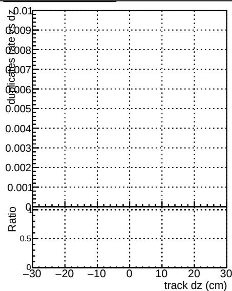
—●— DQM_V0001_R0000000001_Global_CMSSW_orig —●— DQM_V0001_R0000000001_Global_CMSSW_allchi2
