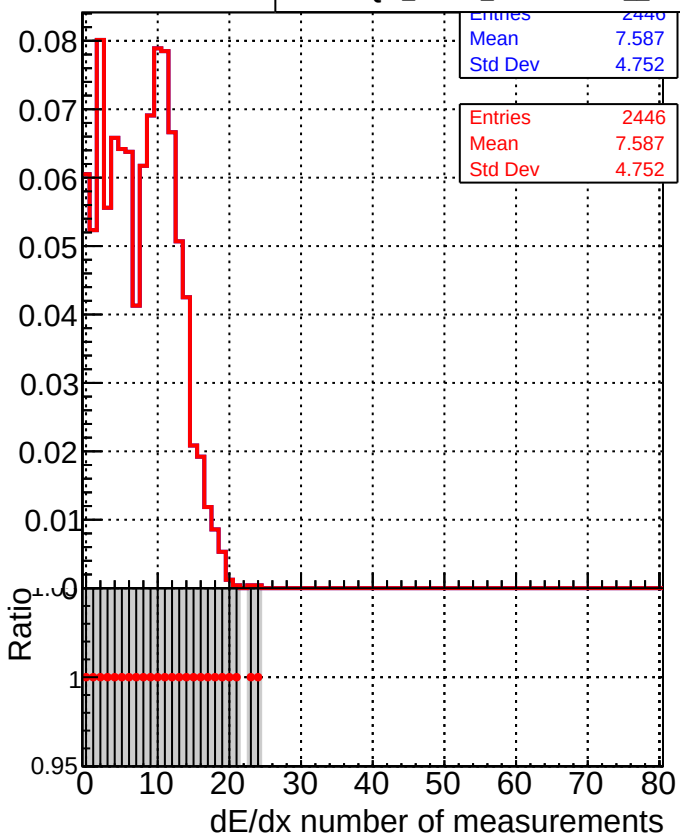
■ DQM_V0001_R000000001_Global_CMSSW_orig ● DQM_V0001_R000000001_Global_CMSSW_allchi2
