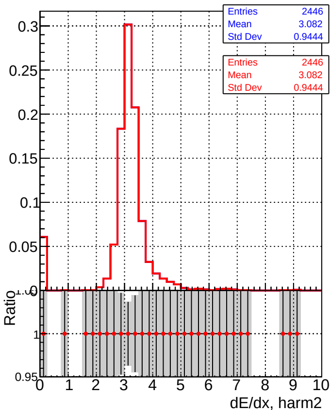
■ DQM_V0001_R000000001_Global_CMSSW_orig ● DQM_V0001_R000000001_Global_CMSSW_allchi2
