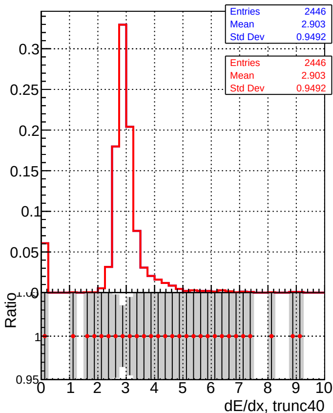
■ DQM_V0001_R000000001_Global_CMSSW_orig ● DQM_V0001_R000000001_Global_CMSSW_allchi2
