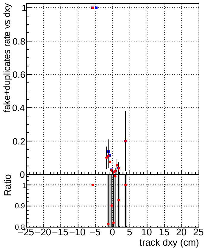
DQM_V0001_R0000000001_Global_CMSSW_orig DQM_V0001_R0000000001_Global_CMSSW_allchi2
