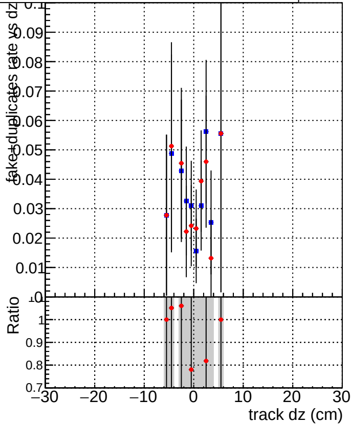
DQM_V0001_R0000000001_Global_CMSSW_orig DQM_V0001_R0000000001_Global_CMSSW_allchi2
