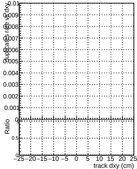
al__CMSSW_orig al__CMSSW_allchi2
