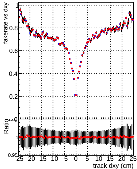
Fake rate vs d —●— DQM_V0001_R0000000001 Global CMSSW_orig —●— DQM_V0001_R0000000001 Global CMSSW_allchi2
