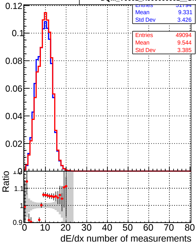
DQM_V0001_R000000001_Global_CMSSW_orig DQM_V0001_R000000001_Global_CMSSW_allchi2
