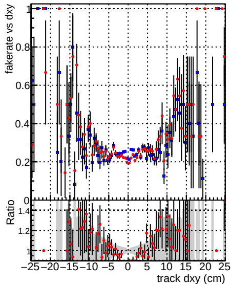
—●— DQM_V0001_R0000000001_Global_CMSSW_orig —●— DQM_V0001_R0000000001_Global_CMSSW_allchi2
