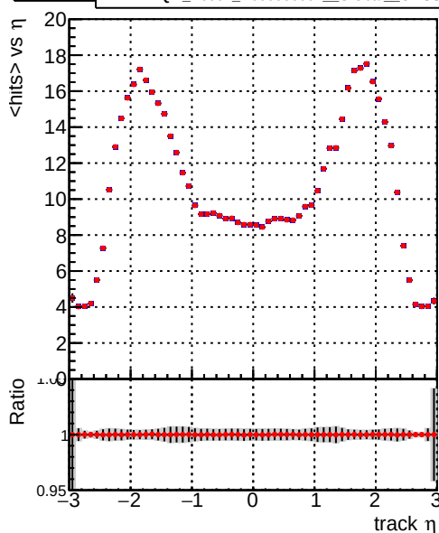
— DQM_V0001_R000000001_Global_CMSSW_orig — DQM_V0001_R000000001_Global_CMSSW_allchi2
