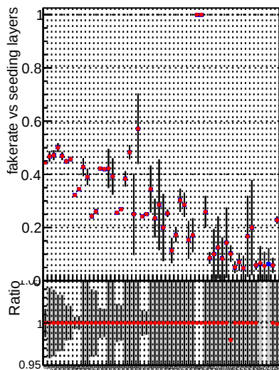
Fake rate vs. —●— DQM_V0001_R0000000001_Global_CMSSW_orig —●— DQM_V0001_R0000000001_Global_CMSSW_allchi2
