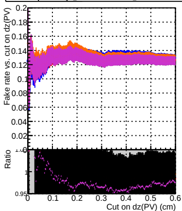
Category Value Real rate 0.05 Fake rate 0.05
