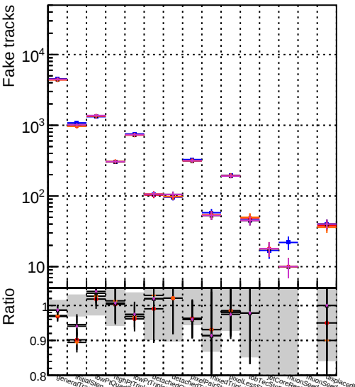
Number Legend Model 1 Black line with triangle DOM mkFitREFit-OR-test_1000evt 2 Orange line with cross DOM mkFitREFit-ORK-test_1000evt 3 Purple line with cross DOM mkFitREFit-OR4-test_1000evt
