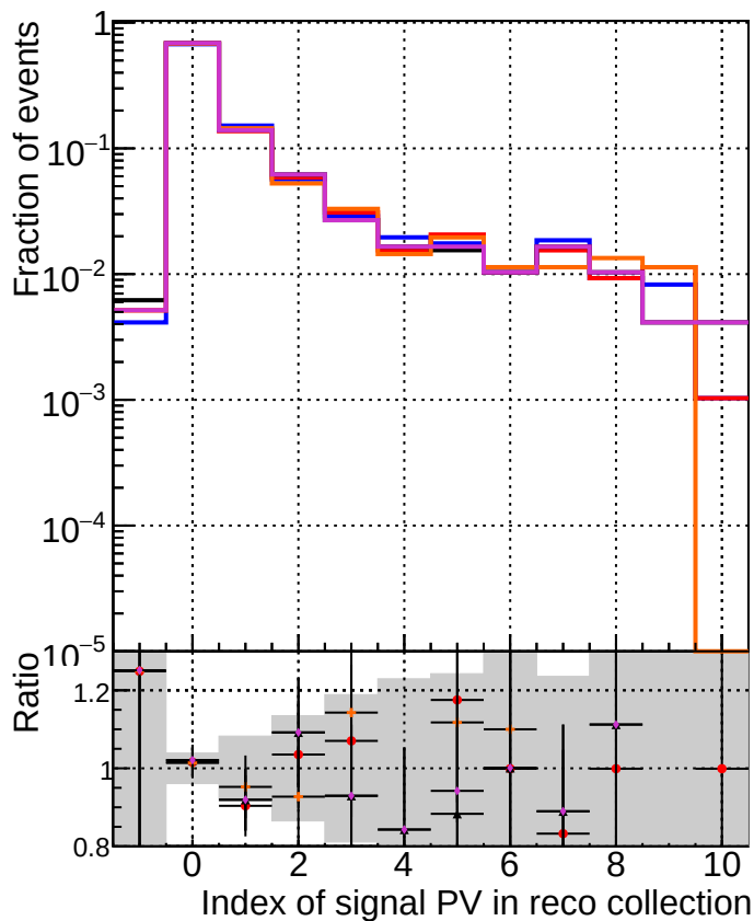
TruePVLocationIndexInRecoVertexCollection
