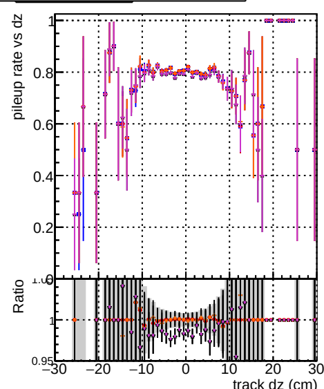
Pileup rate vs dzz
