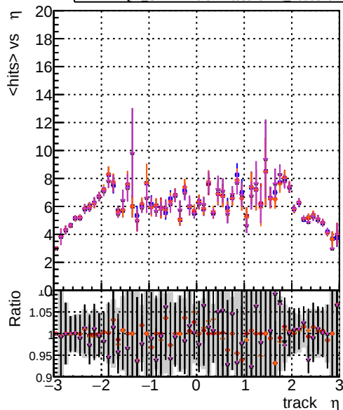
mean hits vs \eta DOM CKF-fit-LowPt_1000evt DOM CKF-fit-LowPt_1000evt DOM CKF-fit-LowPt_1000evt DOM CKF-fit-LowPt_1000evt DOM CKF-fit-LowPt_1000evt
