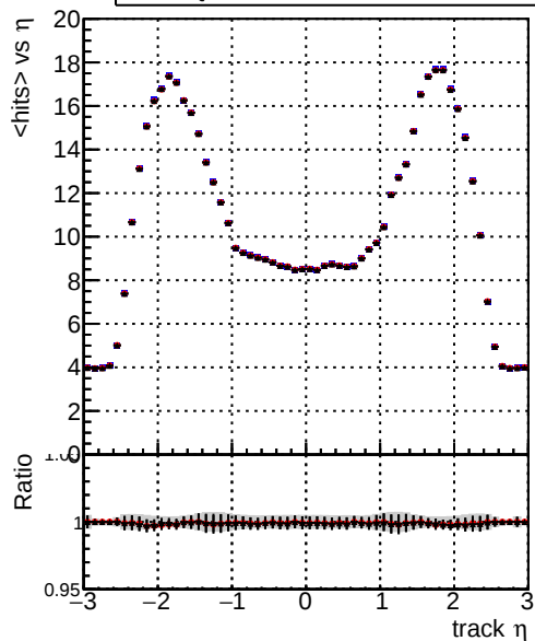
mean hits vs \eta Legend: DQM_TT_CKF_ORIG (blue line) DQM_TT_CKFandPLess_ORIG (red line) DQM_TT_CKFandPLess_MODIF (black line)
