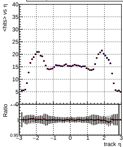
mean hits vs \eta Legend: DQM_TT_CKF_ORIG (blue), DQM_TT_CKFandPLess_ORIG (red), DQM_TT_CKFandPLess_MODIF (black)
