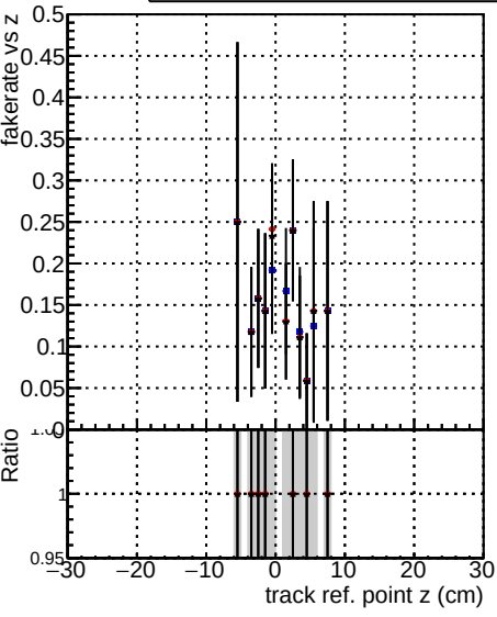
Fake rate vs v DOM_TT_CKF_ORIG DOM_TT_CKFandPLeSS_ORIG DOM_TT_CKFandPLeSS_MODIF
