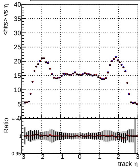
mean hits vs \eta Legend: DQM_TT_CKF_ORIG (blue), DQM_TT_CKFandPLess_ORIG (red), DQM_TT_CKFandPLess_MODIF (black)
