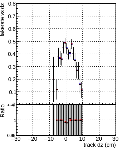
Fake rate vs dz Legend: DOM TT CKF ORIG DOM TT CKFandPless ORIG DOM TT CKFandPless MODIF
