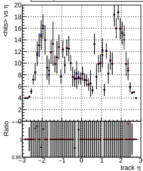
mean hit Legend: DQM_TT_CKF_ORIG (blue), DQM_TT_CKFandPless_ORIG (red), DQM_TT_CKFandPless_MODIF (black)
