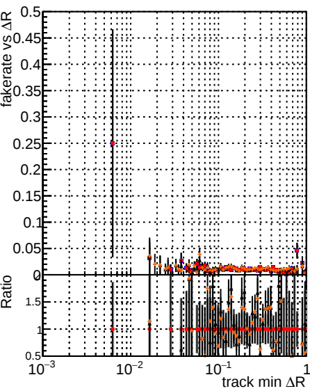
Fake rate vs ΔR(track, jet) for different methods: DOM, XMinus, original, newbranch, original pless, newbranch pless
