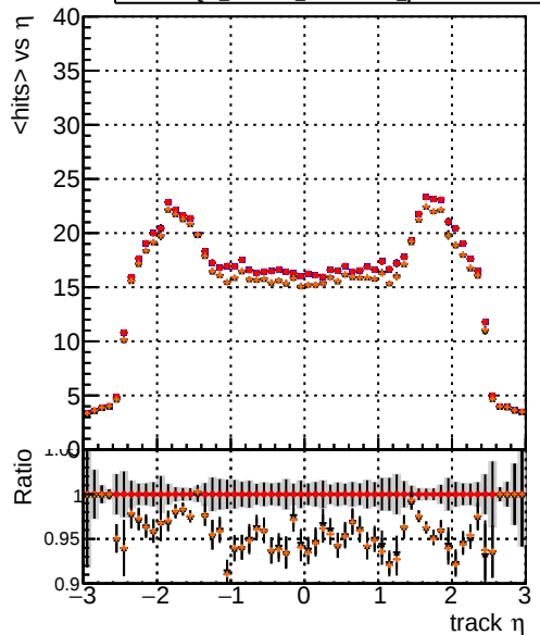
Legend: DQM_XiMinus_original (blue line), DQM_XiMinus_newbranch (red line), DQM_XiMinus_original_pLess (black line), DQM_XiMinus_newbranch_pLess (orange line) mean hits vs \eta
