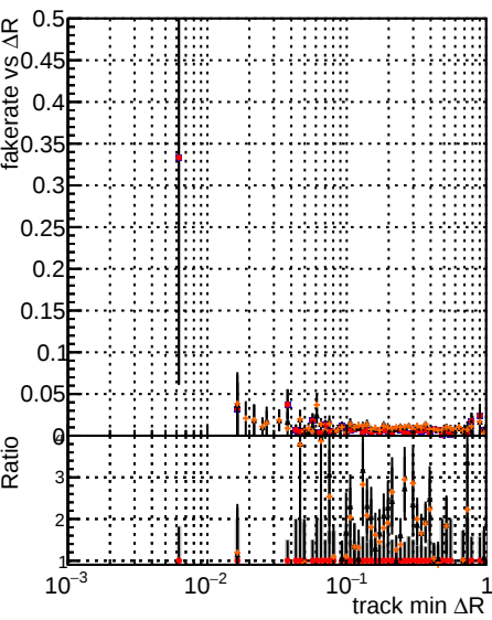
Fake rate vs ΔR(track, jet) for different models and methods Model Method Color Shape DQM XiMinus original Blue Square XiMinus newbranch Red Triangle DQM XiMinus original pless Black Circle XiMinus newbranch pless Orange Star
