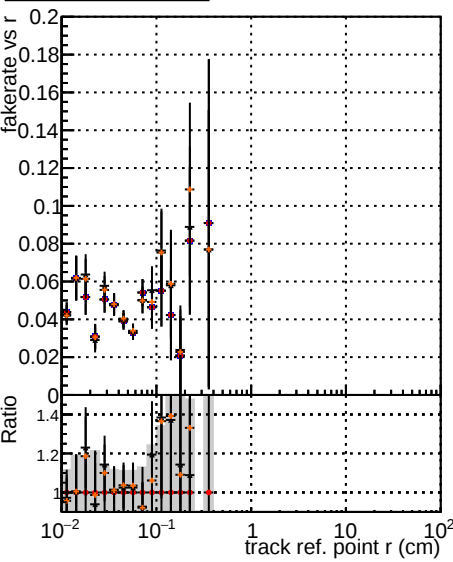
Fake rate vs verpos Legend: - original (black line) - newbranch (red line) - newbranch pless (orange line)
