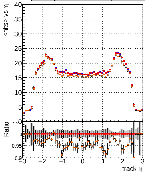
mean hits vs \eta — DQM_XiMinus_original — DQM_XiMinus_newbranch — DQM_XiMinus_original_pLess — DQM_XiMinus_newbranch_pLess
