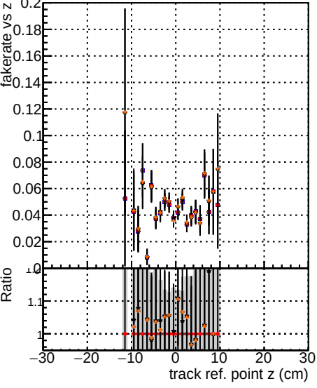
Fake rate vs verpos Legend: original (black line with dots) newbranch (red line with dots) newbranch pless (orange line with dots)
