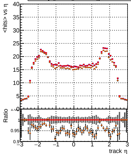
mean hits vs \eta Legend: DQM_XiMinus_original (blue line), DQM_XiMinus_newbranch (red line), DQM_XiMinus_original_pLess (black line with error bars), DQM_XiMinus_newbranch_pLess (orange line with error bars)
