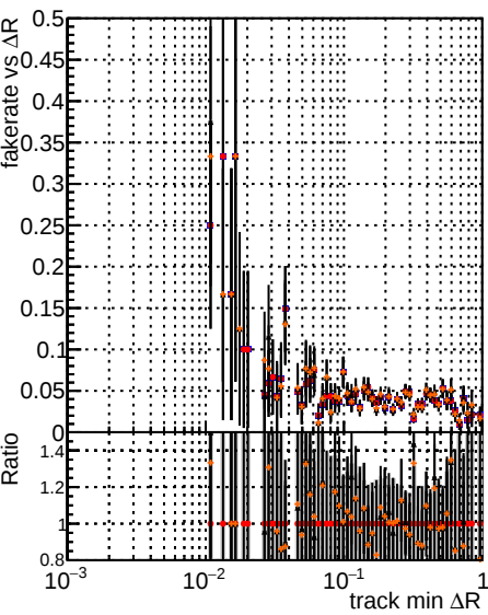
Fake rate vs \Delta R(\text{track}, \text{jet}) Legend: original (black line) newbranch (red line) original plus (orange line)
