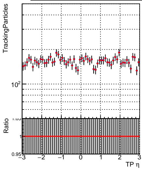
Legend: DQM_TT_time_newbranch (blue dots), DQM_TT_newbranch_time_pLess (red dots)
