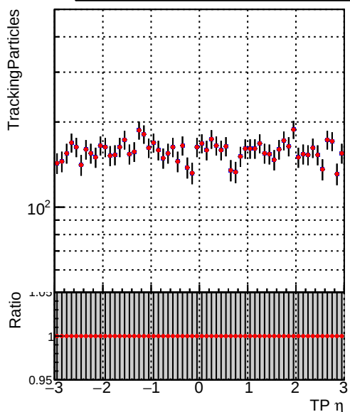
Legend: \blacksquare DQM_TT_time_newbranch \bullet DQM_TT_newbranch_time_pLess
