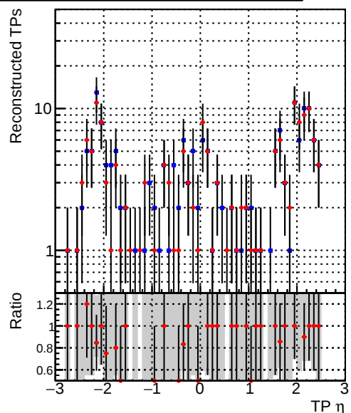
Legend: \blacksquare DQM_TT_time_newbranch \bullet DQM_TT_newbranch_time_pLess
