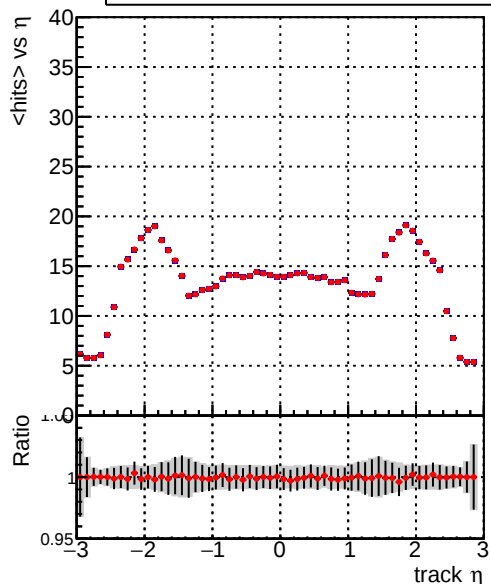
mean hits vs \eta Legend: DQM_TT_time_newbranch (blue line), DQM_TT_newbranch_time_pLess (red line)
