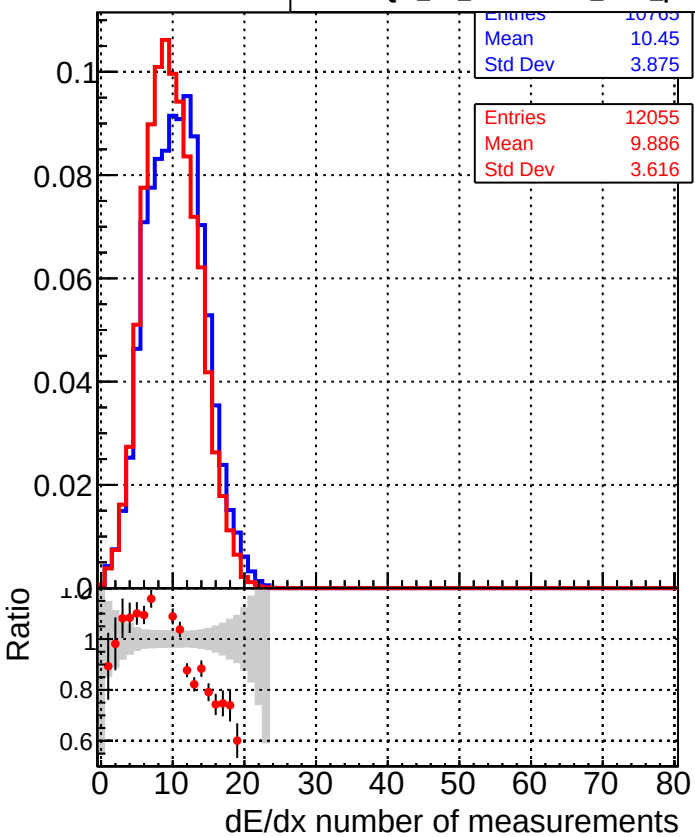
— DQM_TT_time_newbranch — DQM_TT_newbranch_time_pLess
