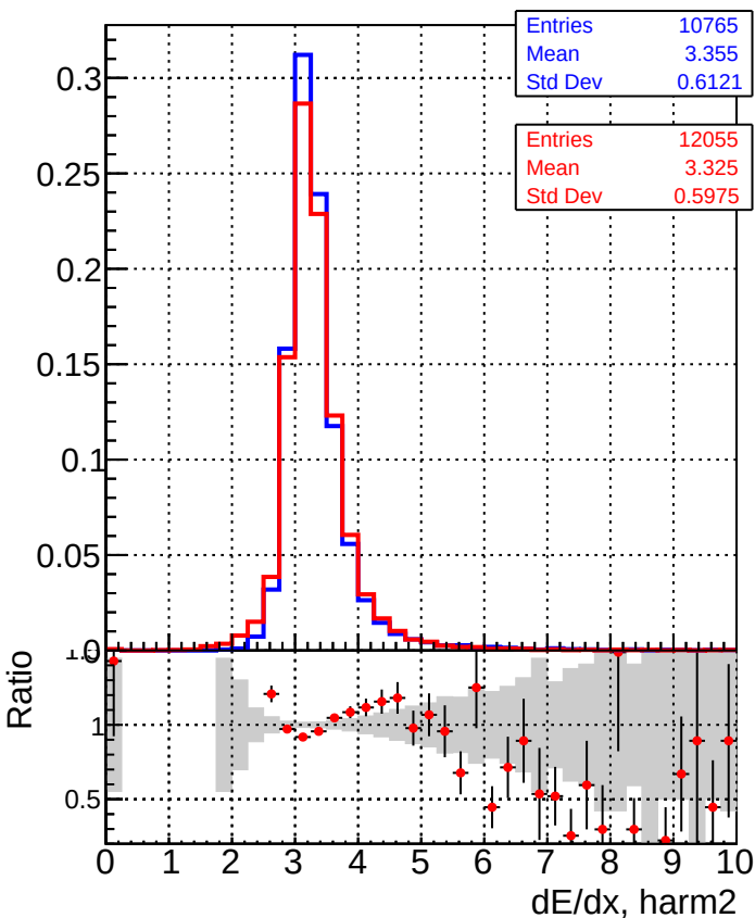
— DQM_TT_time_newbranch — DQM_TT_newbranch_time_pLess
