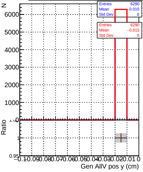
GeneratedAllV_Y DQM_TT_time_newbranch DQM_TT_newbranch_time_pLess
