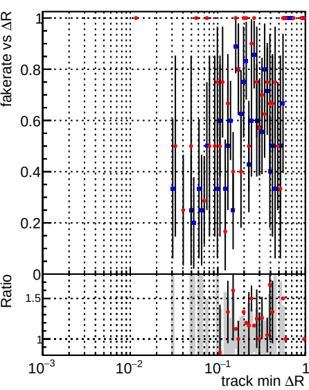
Fake rate vs \Delta R(\text{track, jet}) Legend: DQM_TT_time_newbranch (blue dots), DQM_TT_newbranch_time_pLess (red dots)
