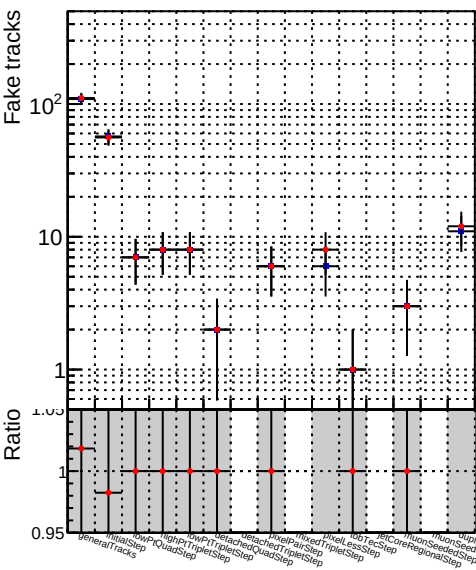
Number —●— DQM_TT_newbranch_time_pLess
