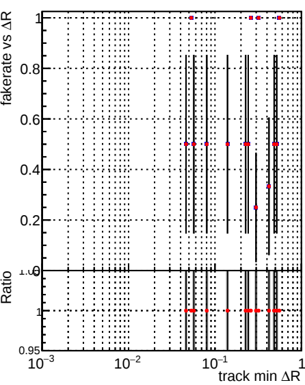
Fake rate vs ΔR(track, jet) DQM_TT_time_newbranch DQM_TT_newbranch_time_pLess
