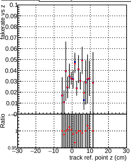
—•— DQM_TT_time_newbranch —•— DQM_TT_newbranch_time_pLess
