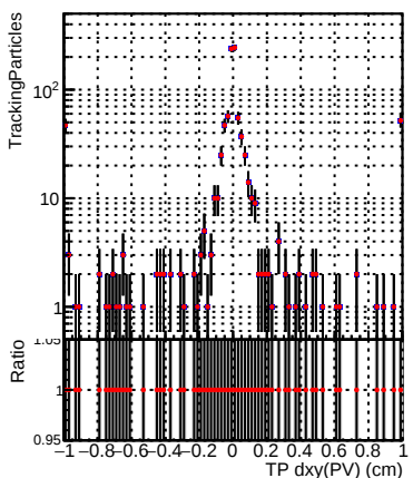
N of sim — DQM_TT_newbranch_t
