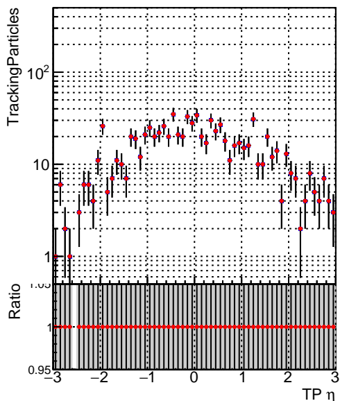
N of simulated tracks vs TP η ■ DQM_TT_time_newbranch ● DQM_TT_newbranch_time_pLess
